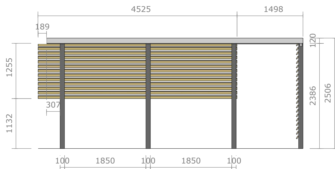
PERGOLA ELEVATION SCALE 1: 50 @ A1
