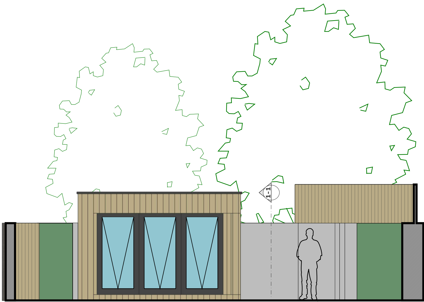
SECTION 2-2 SCALE 1: 50 @ A1
