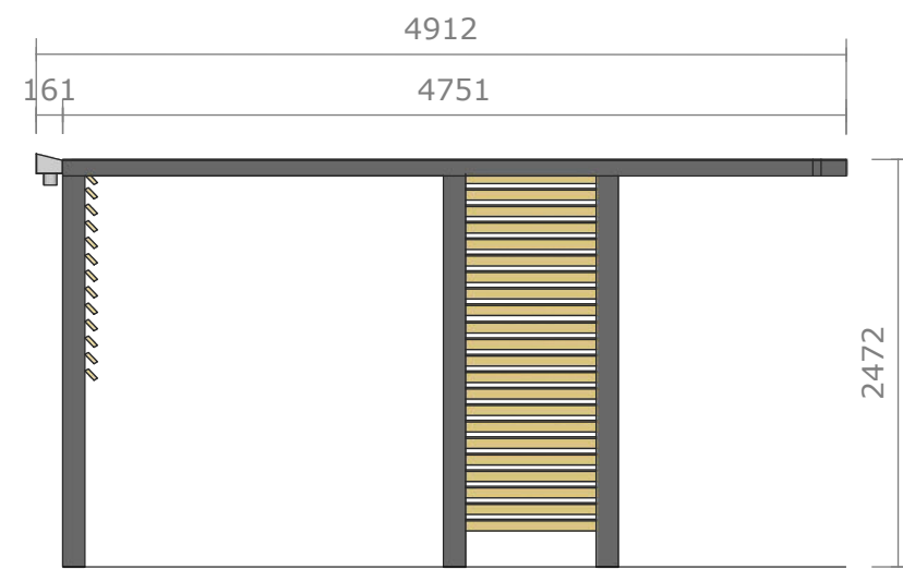
PERGOLA END ELEVATION SCALE 1: 50 @ A1
