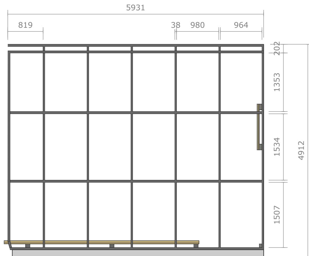
PERGOLA PLAN VIEW SCALE 1: 50 @ A1
