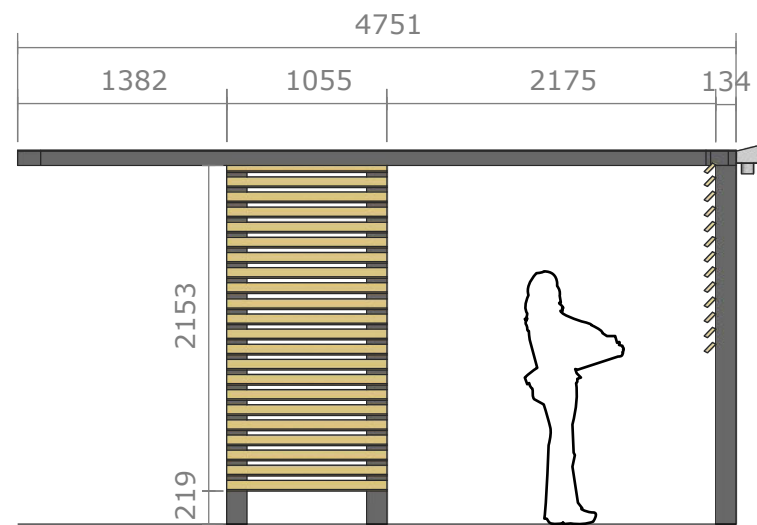
PERGOLA END ELEVATION SCALE 1: 50 @ A1
